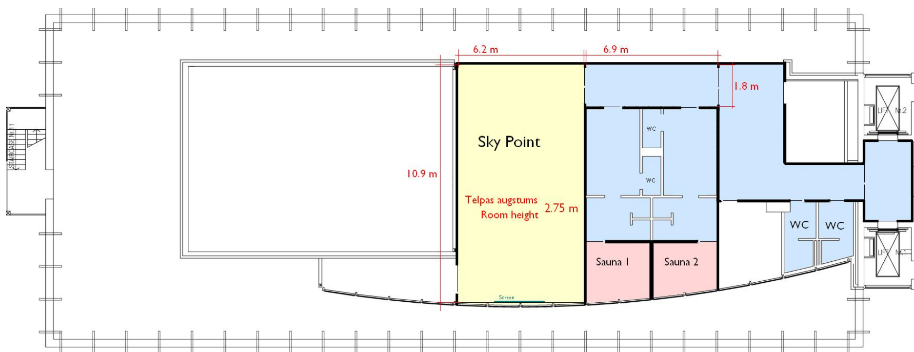
27 FLOOR PLAN
